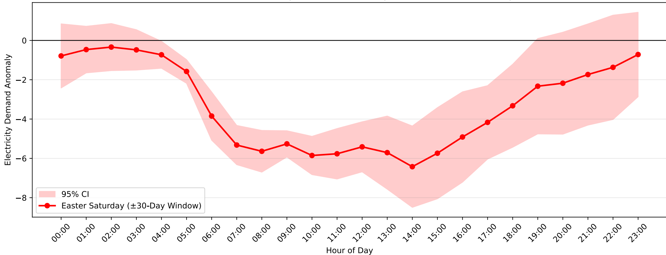
Bankstown Demand Anomaly: Easter Saturday (2015-2016, \pm 30 -Day Window)
