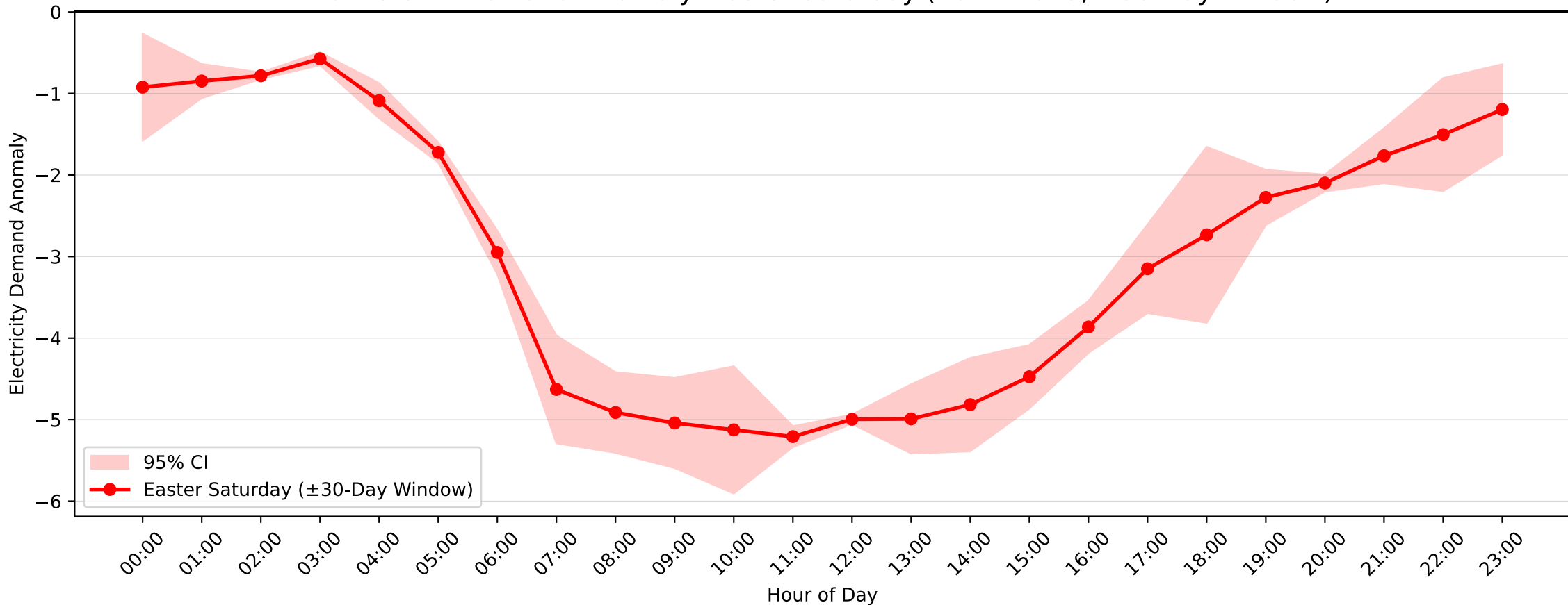
Bankstown Demand Anomaly: Easter Saturday (2012-2013, \pm 30 -Day Window)
