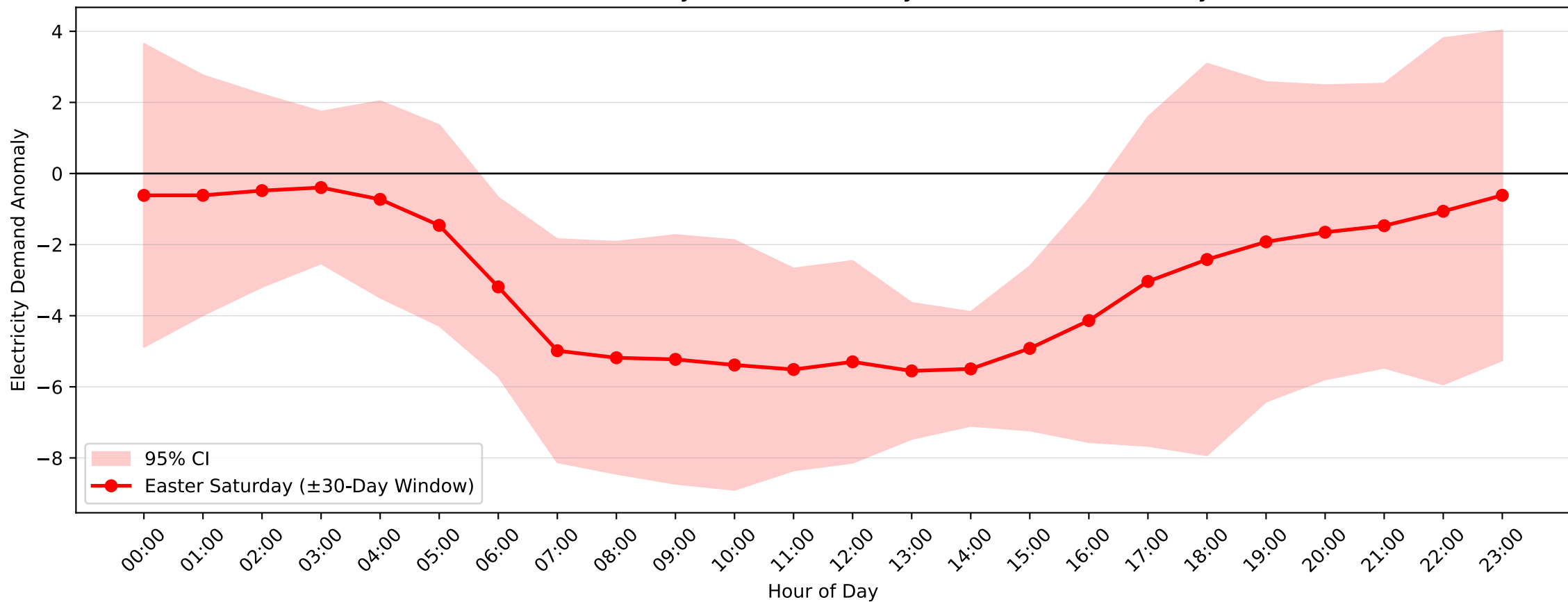
Bankstown Demand Anomaly: Easter Saturday (2013-2014, \pm 30 -Day Window)
