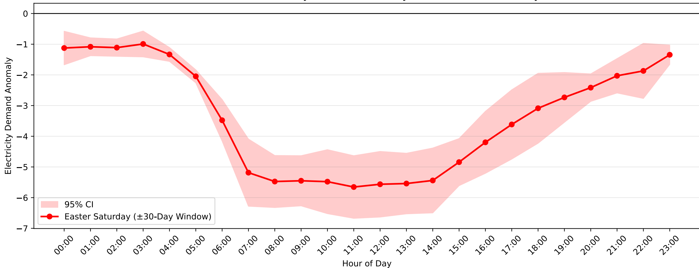
Bankstown Demand Anomaly: Easter Saturday (2011-2012, \pm 30 -Day Window)
